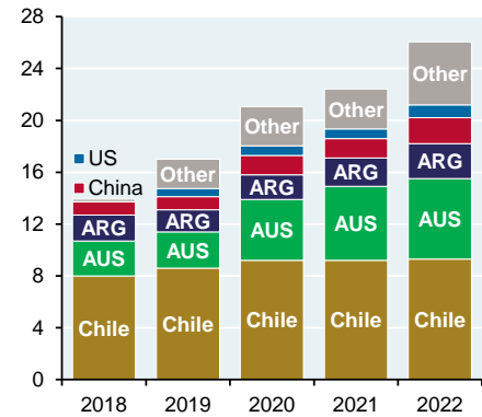
Global reserves of lithium by country Million metric tons
